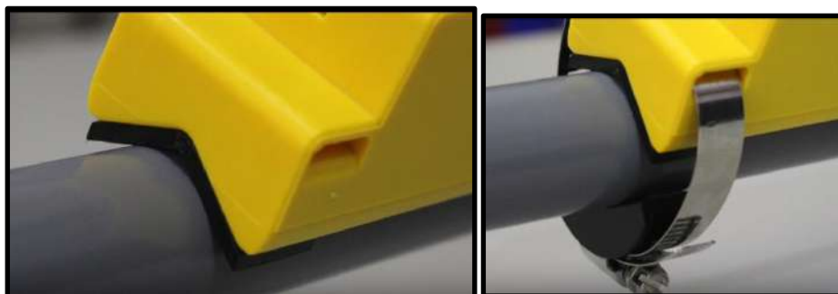
Clamping pipe adaptor to pipe with OD less than 40mm
