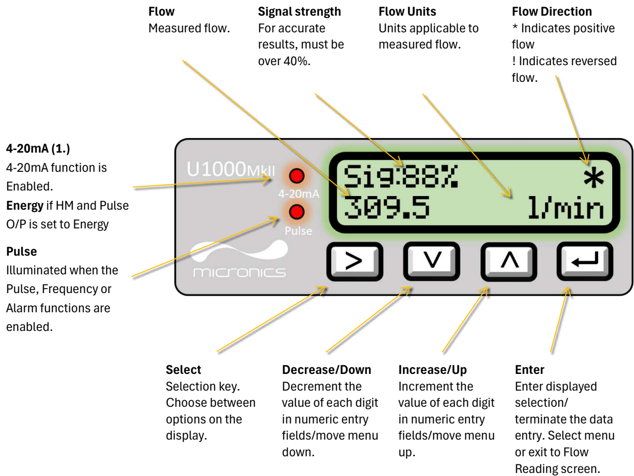
Figure 3 : Display
