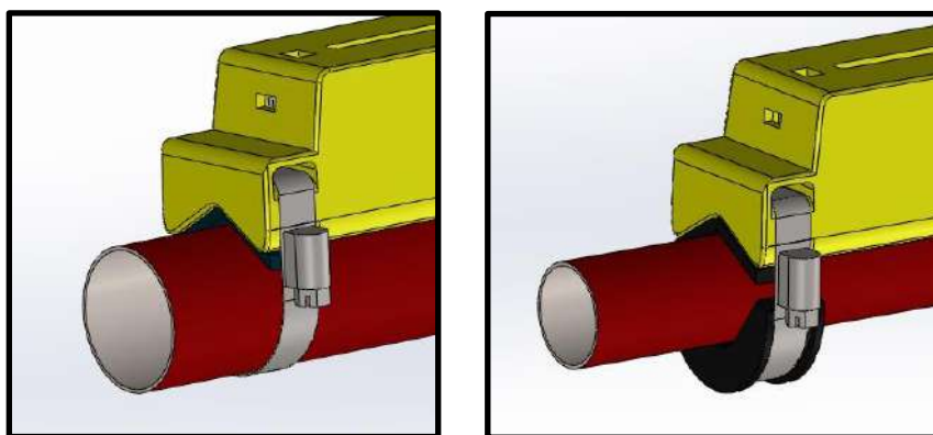
Pipe adaptors in position: 40-60mm OD (left), less than 40mm OD (right)
