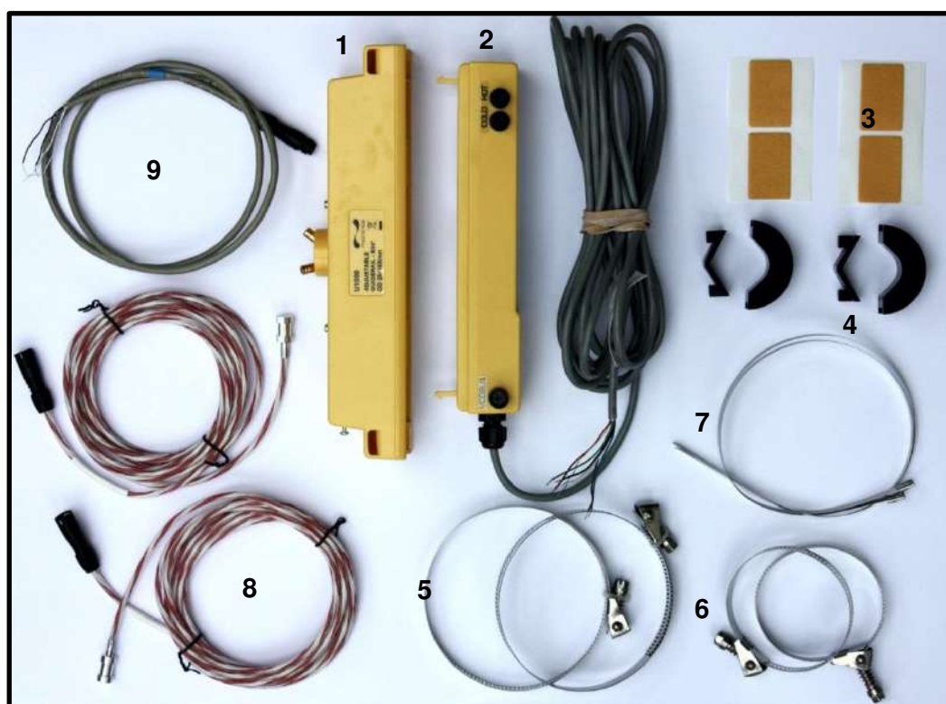
Figure 2 : Package Contents
