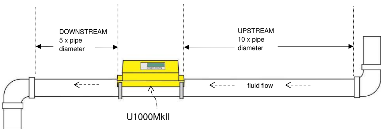
Figure 4 : Recommended Install Location of U1000
