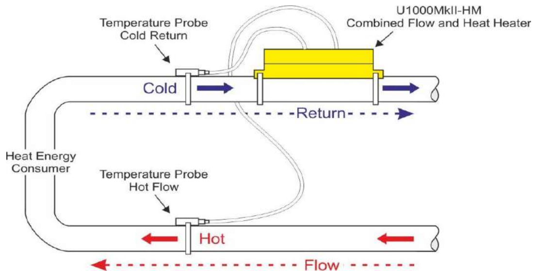
Figure 5 : Location with Temperature Probes
